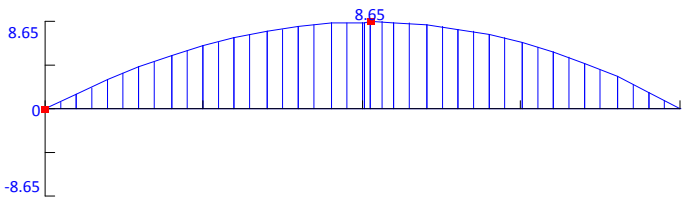
Moment Diagram (Y) (kip-ft)
