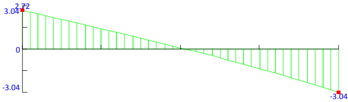
Shear Diagram (X) (kip)
