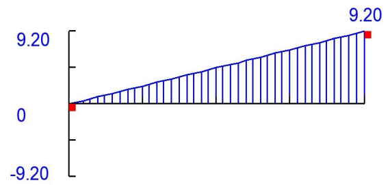
Moment Diagram (X)
