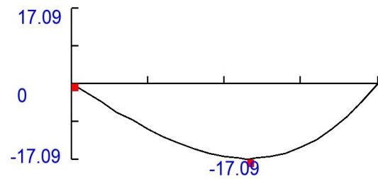
Deflection Diagram (Y) ( 1/100 in )
